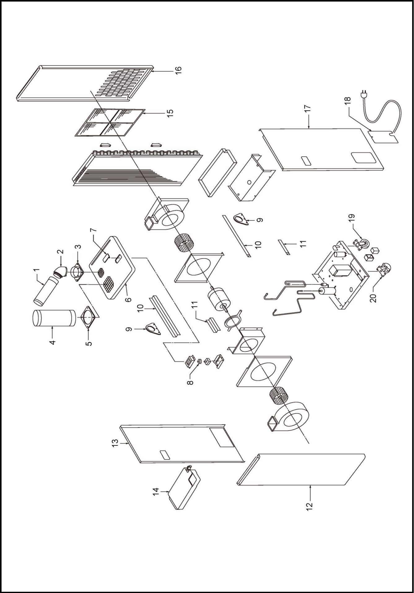
FIG. 1 SPOT COOLER MSC25A, MSC25A-1
